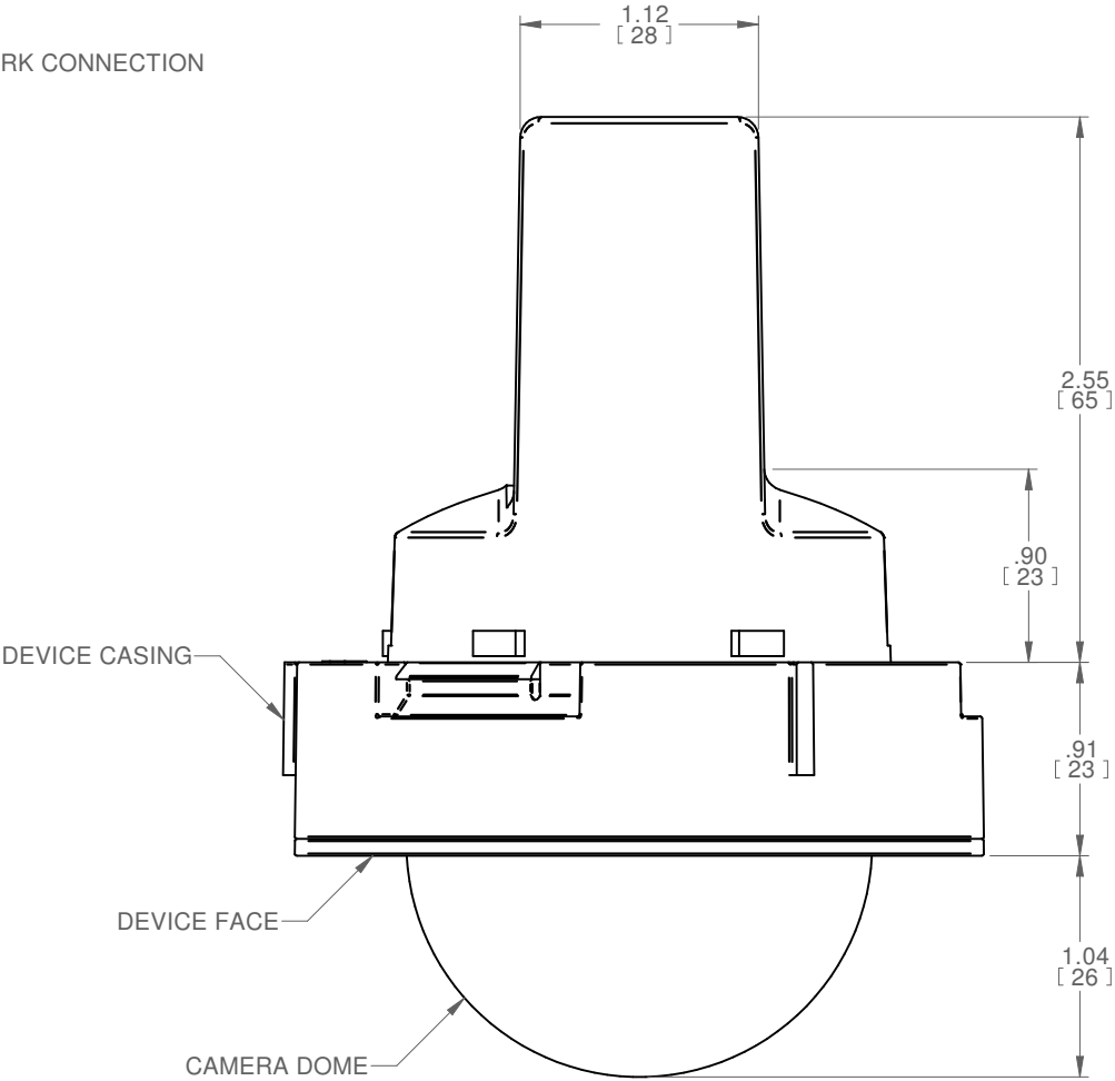
FRONT VIEW
