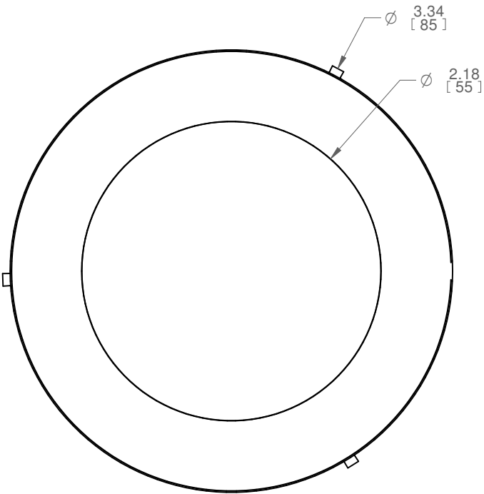
BOTTOM VIEW
